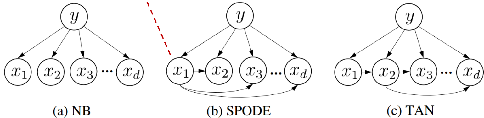
Fig. 7.1: Feature dependencies of naïve Bayes and semi-naïve Bayes classifiers.
